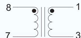
Schematic
